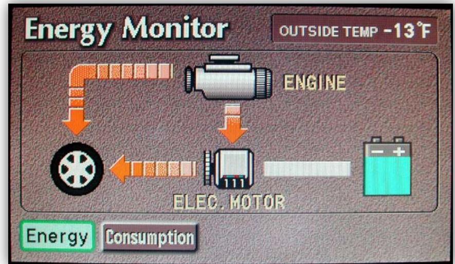
PriusEnergy_EngineMotorDrive_-13Fdegrees_01
