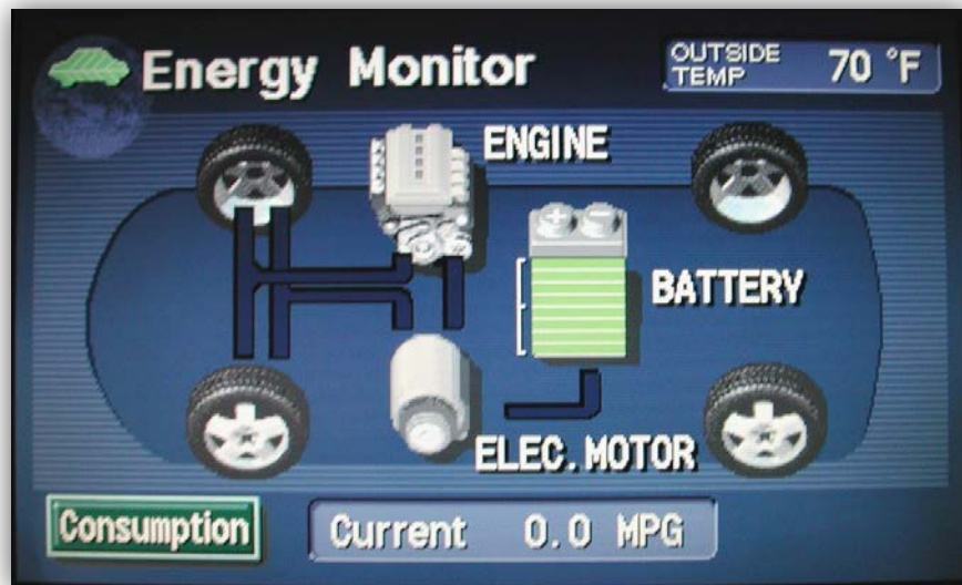
PriusEnergy_Charge-Level_All-Green_01
