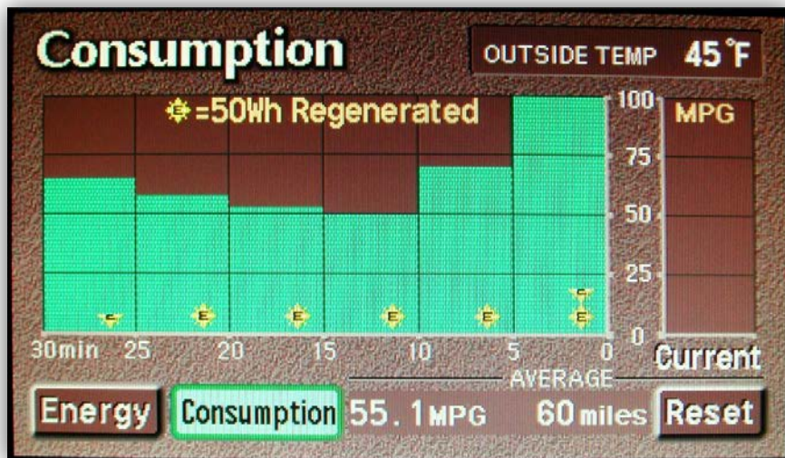
PriusConsumption_MyFinalMorningCommute
