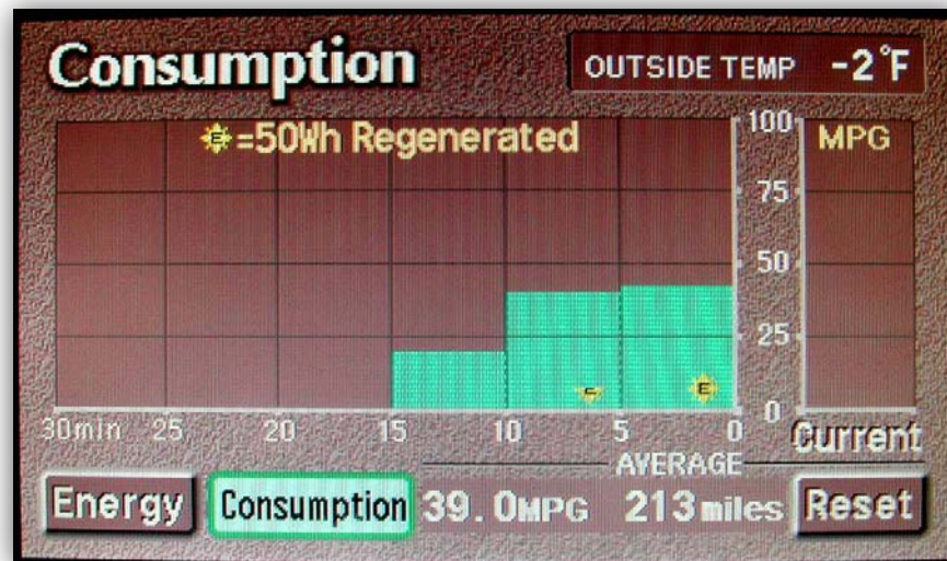
PriusConsumption_CloseUp_-2Fdegrees_01
