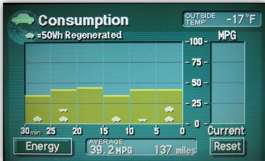
PriusConsumption_ExtremeCold_Green
