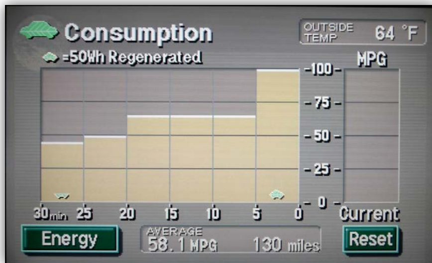
PriusConsumption_CloseUp_58MPG_Beige
